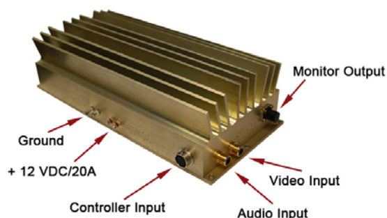
100 W Programmable Video Transmitter from 1.5 -2.5 GHz
